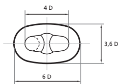
COMMON LINK
