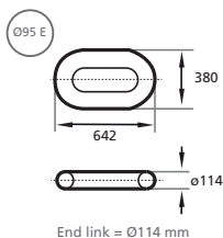
End link = Ø114 mm
