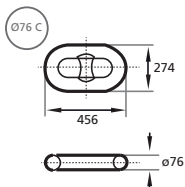
Common Link = Ø76 mm
