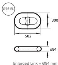
Enlarged Link = Ø84 mm
