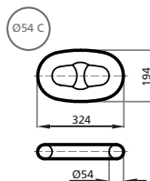
COMMON LINK = C (Ø54)
