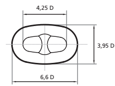
ENLARGED LINK
