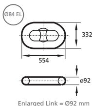
Enlarged Link = Ø92 mm
