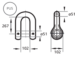
Pick Up Shackle = PUS
