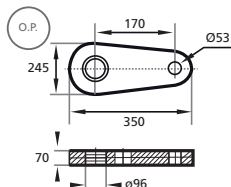
Oblong plate = OP
